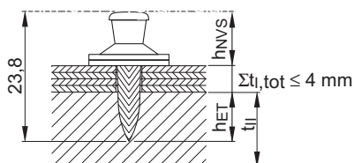
Siding and decking pin X-ENP-19 L15
