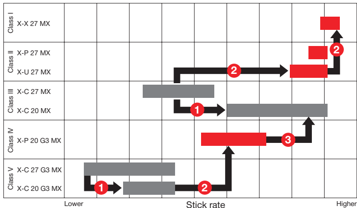
Indicative stick rate ranges per nail class in tough concrete
